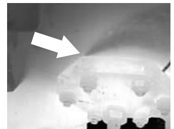
The sniffer is detecting gas but unable to trace its source, whereas this thermal image shows the leak source clearly on the left.
